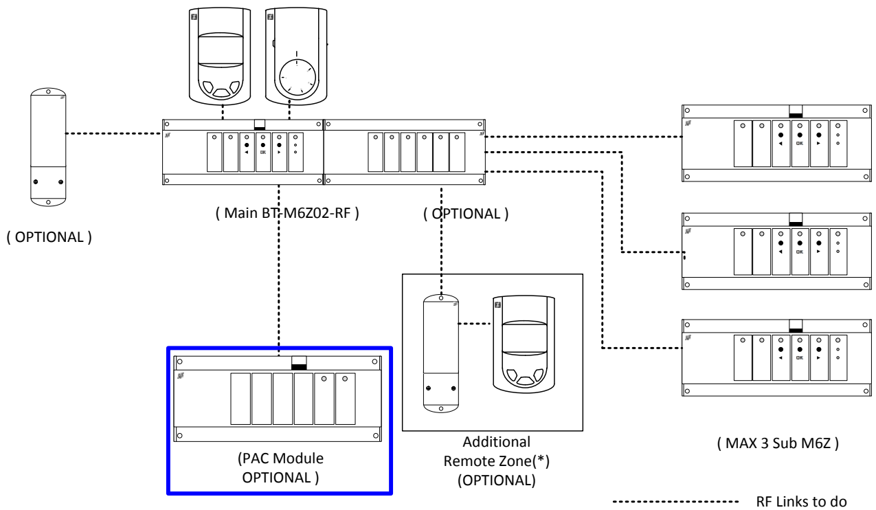
Installation without BT-CT02-RF
